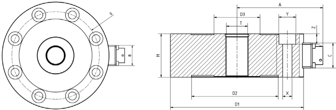
Dimensional drawing
